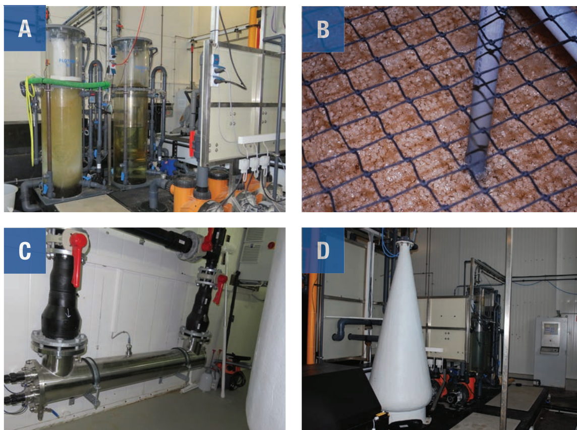
Figure 18. Equipment for water treatment at an RAS facility. (A) Protein skimmers remove loose organic matter (B) Bacteria grow in a moving bed biofilm reactor (MBBR) as a biofilm on a substrate that increases the surface area (plastic balls are used here). Biofilm covers a large surface area over the water and breaks down and treats the water to remove substances containing nitrogen (that are toxic to farming organisms) from the water. (C) Disinfection. The water passes a UV lamp emitting light with a wavelength of 254 nm in order to remove viruses, bacteria, fungi and parasites. (D) Oxygenation of the water. Pure oxygen under pressure is added to the water in an oxygen concentrator.
